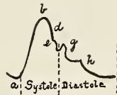
FIG. 130.—The normal radial curves: a-b , the tidal wave; b-e , the aortic notch; d , the dirotic wave; h , the post-dirotic wave.
